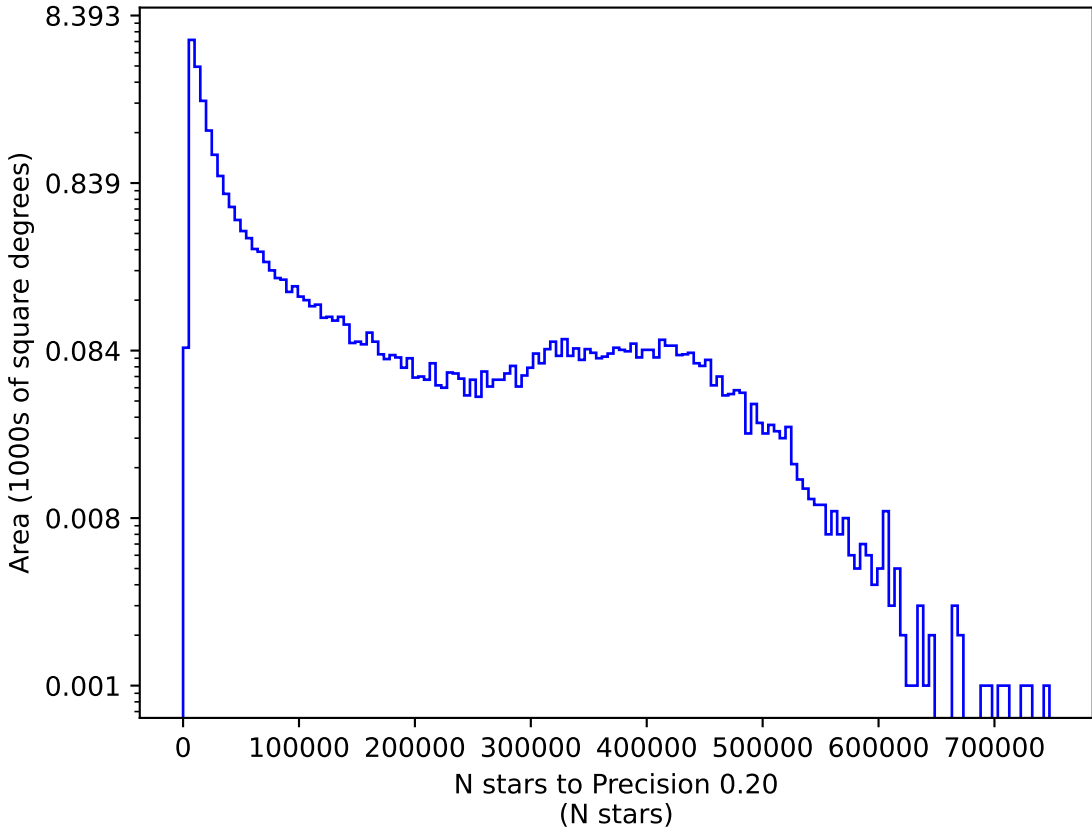
ddf_acor_sf25_lsf30_lsr50_v3.4_10yrs z: N stars to Precision 0.20
