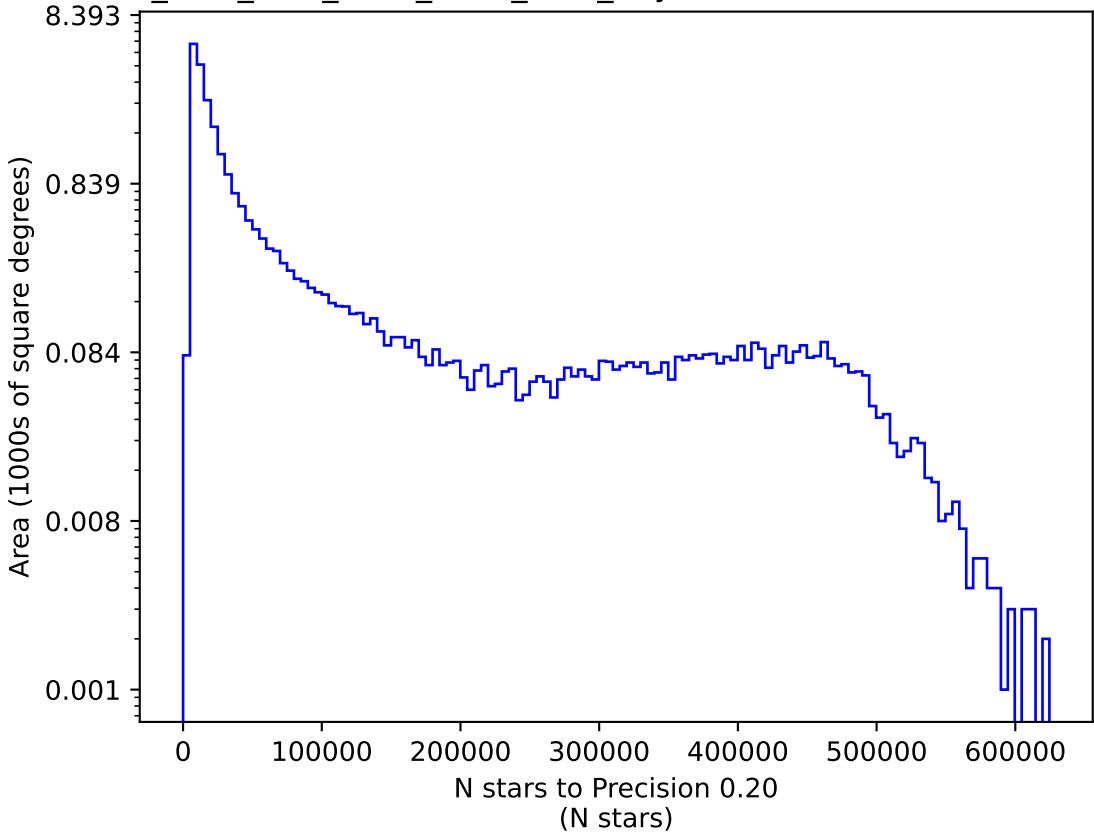
ddf_acor_sf25_lsf30_lsr50_v3.4_10yrs i: N stars to Precision 0.20
