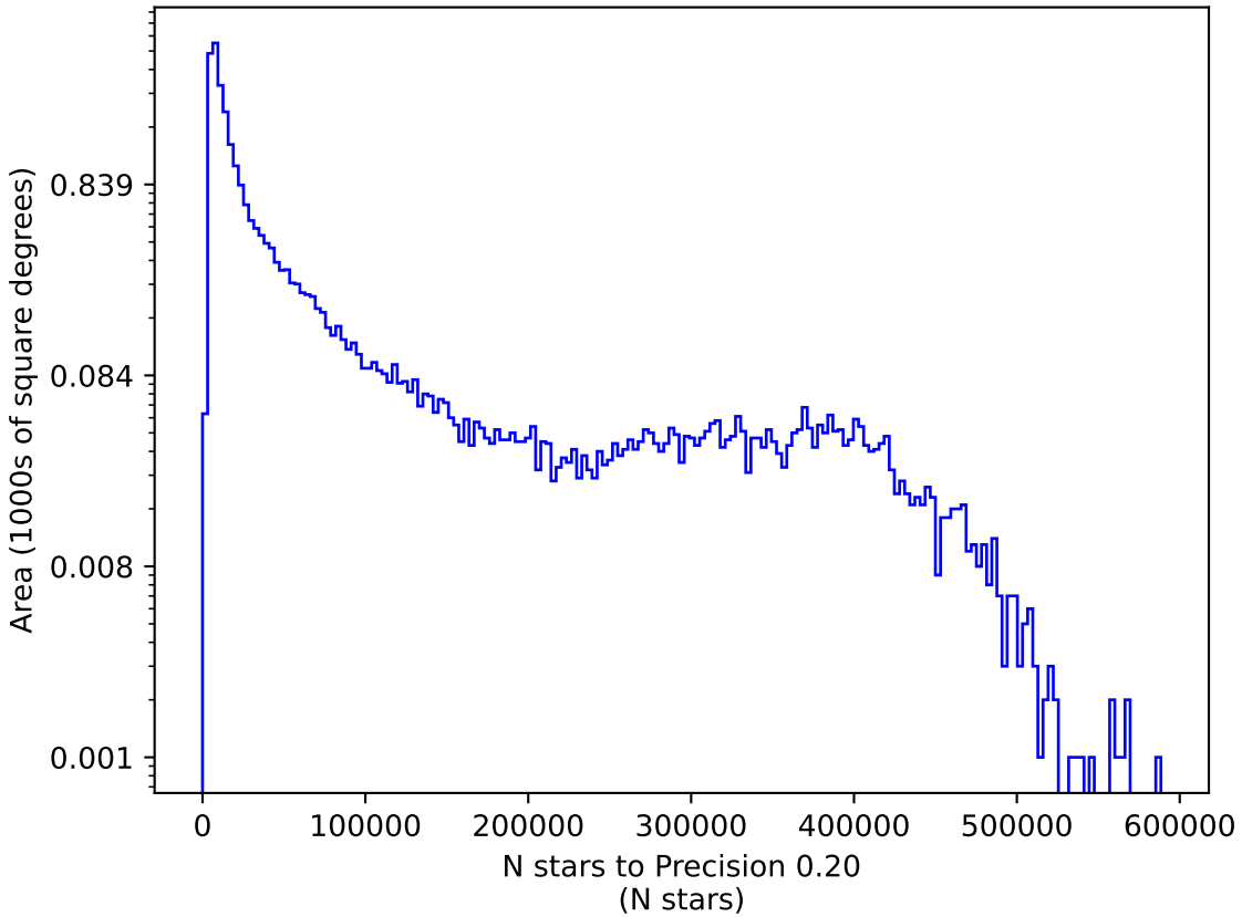
ddf_acor_sf25_lsf30_lsr50_v3.4_10yrs g: N stars to Precision 0.20
