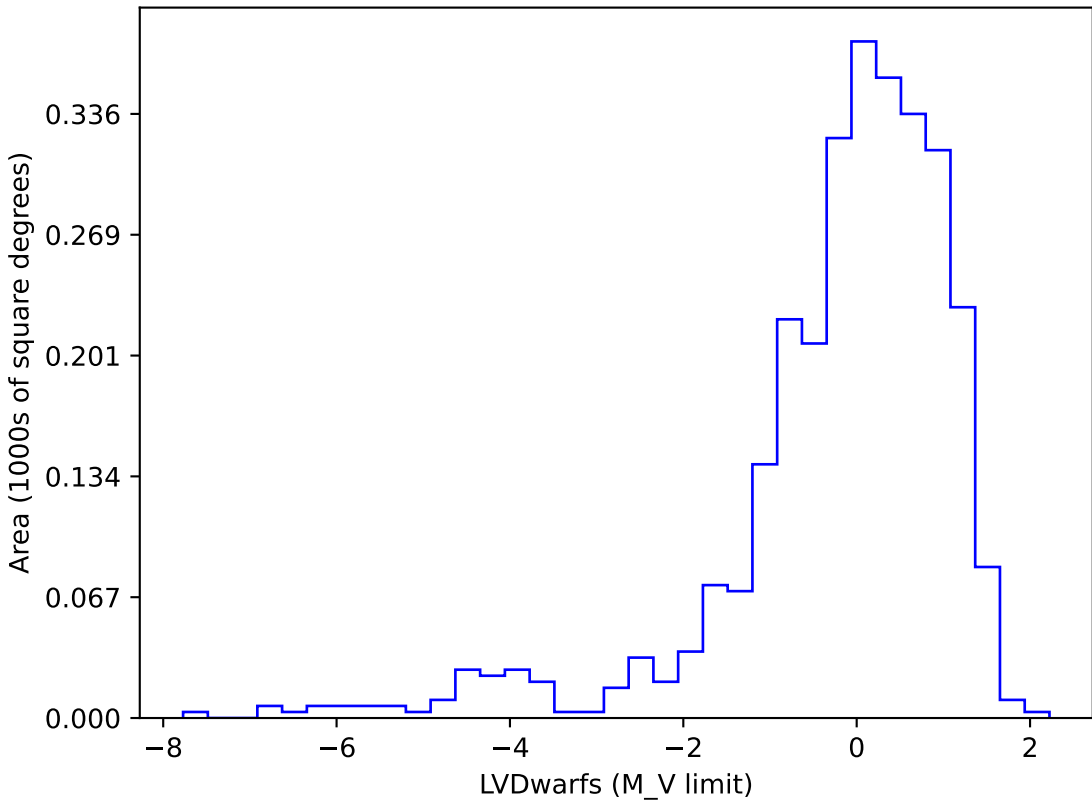
ddf_acor_sf25_lsf30_lsr50_v3.4_10yrs gi SCP: LVDwarfs
