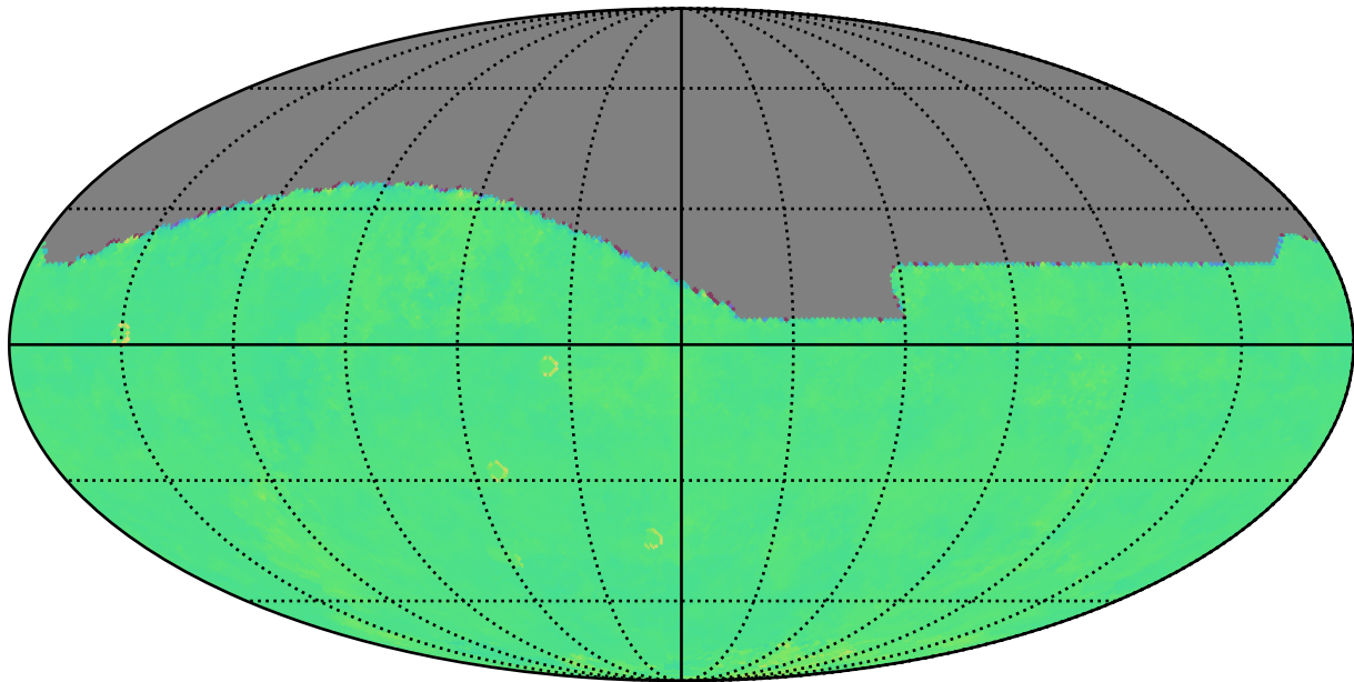
ddf_acor_sf25_lsf30_lsr50_v3.4_10yrs r: Kuiper rotTelPos
