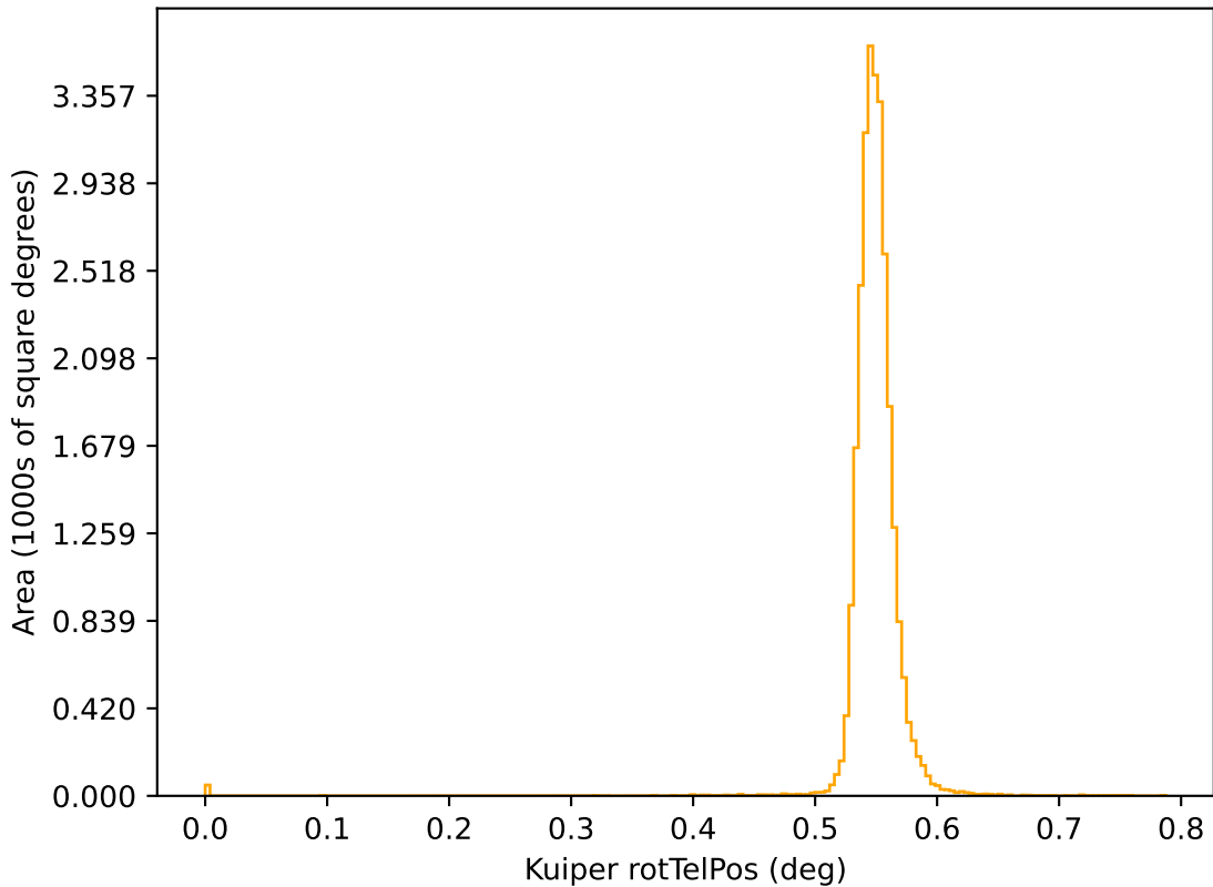
ddf_acor_sf25_lsf30_lsr50_v3.4_10yrs r: Kuiper rotTelPos
