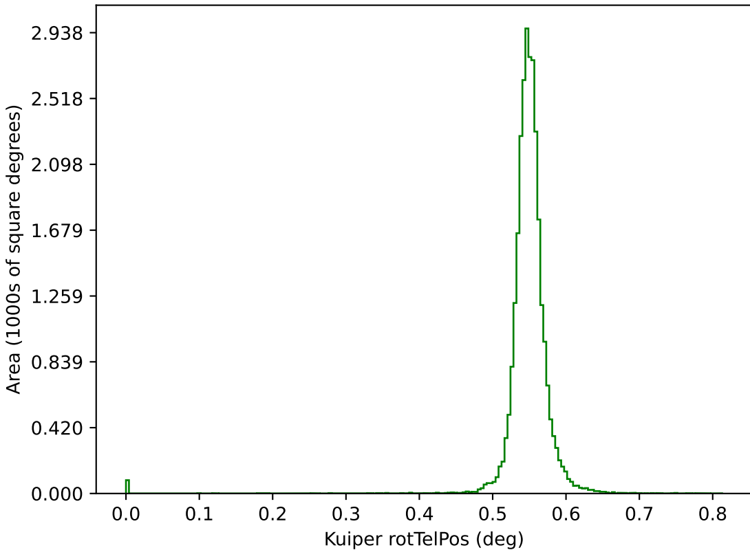
ddf_acor_sf25_lsf30_lsr50_v3.4_10yrs g: Kuiper rotTelPos
