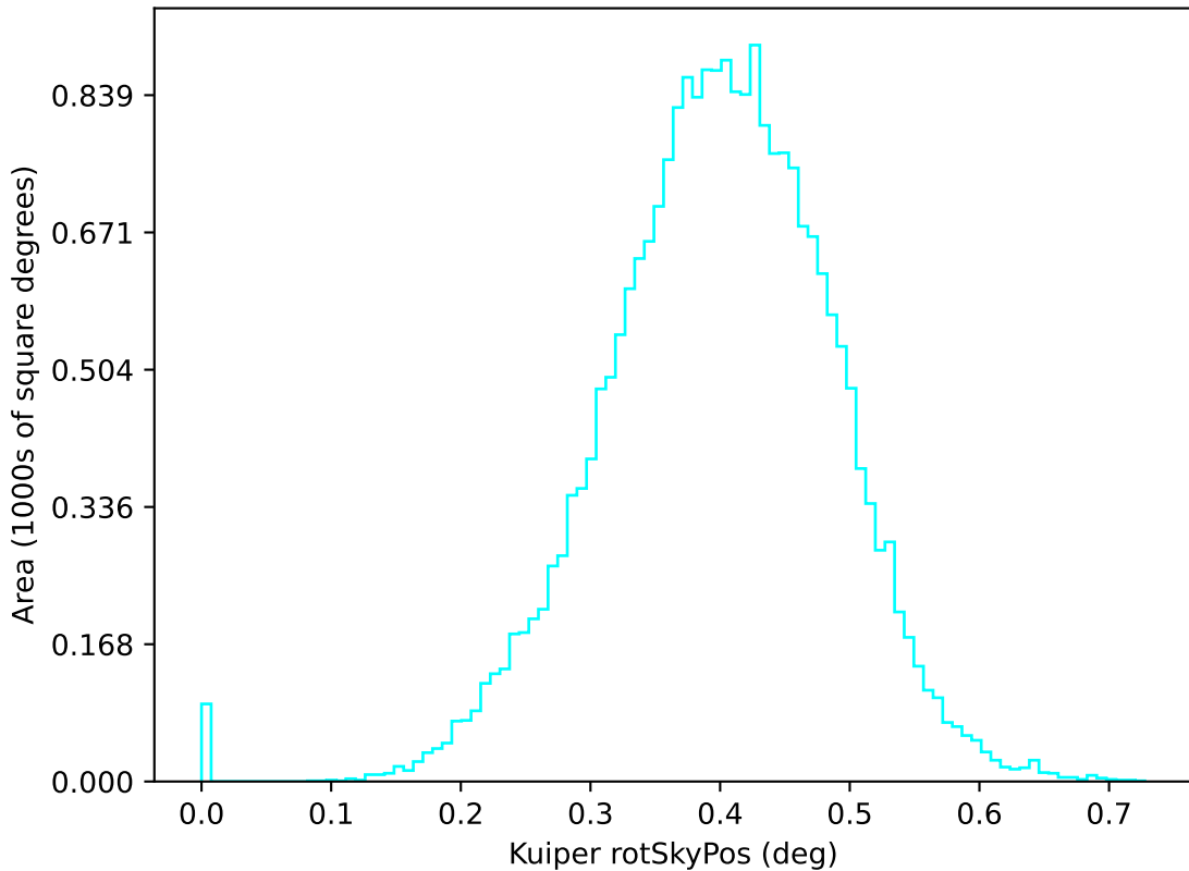
ddf_acor_sf25_lsf30_lsr50_v3.4_10yrs u: Kuiper rotSkyPos
