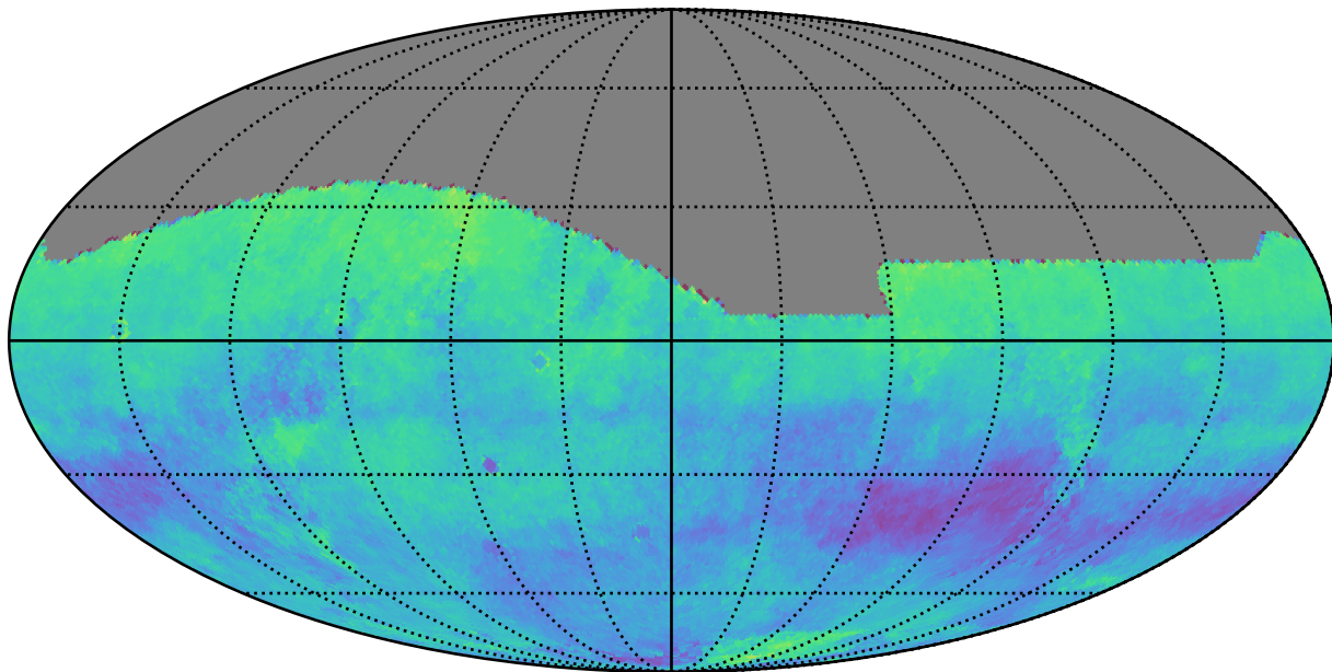
ddf_acor_sf25_lsf30_lsr50_v3.4_10yrs r: Kuiper rotSkyPos
