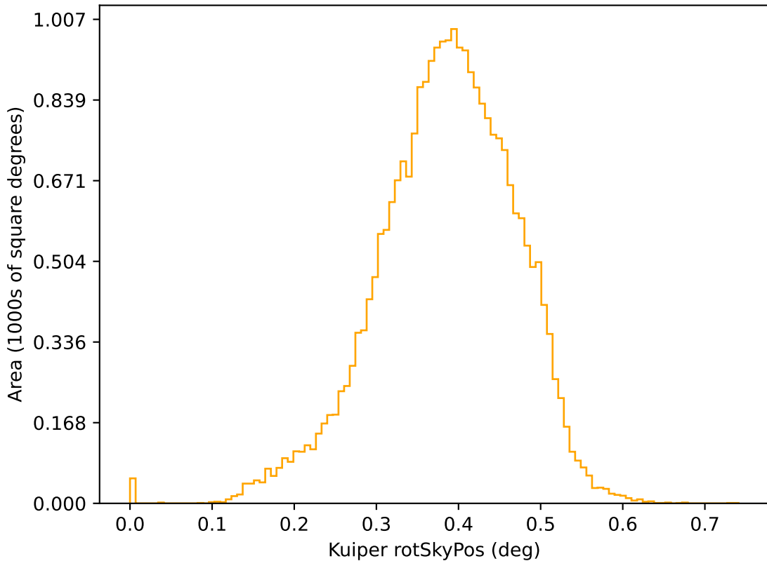
ddf_acor_sf25_lsf30_lsr50_v3.4_10yrs r: Kuiper rotSkyPos
