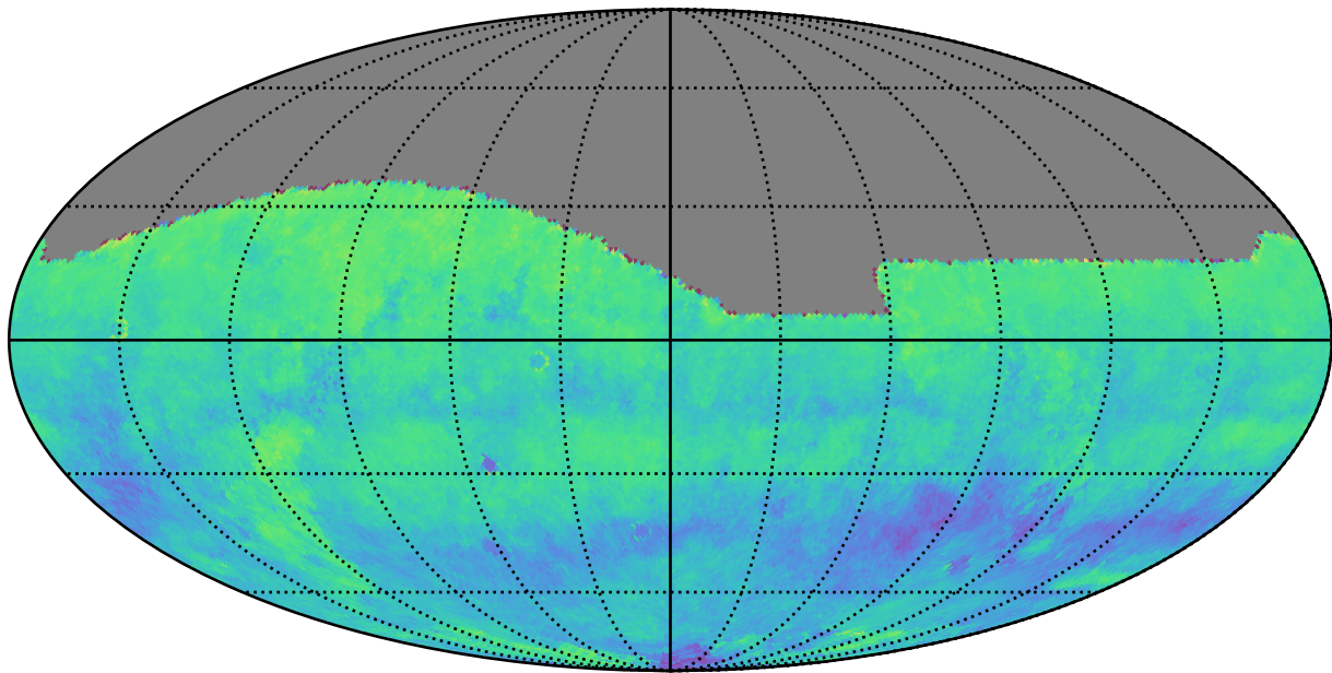
ddf_acor_sf25_lsf30_lsr50_v3.4_10yrs i: Kuiper rotSkyPos
