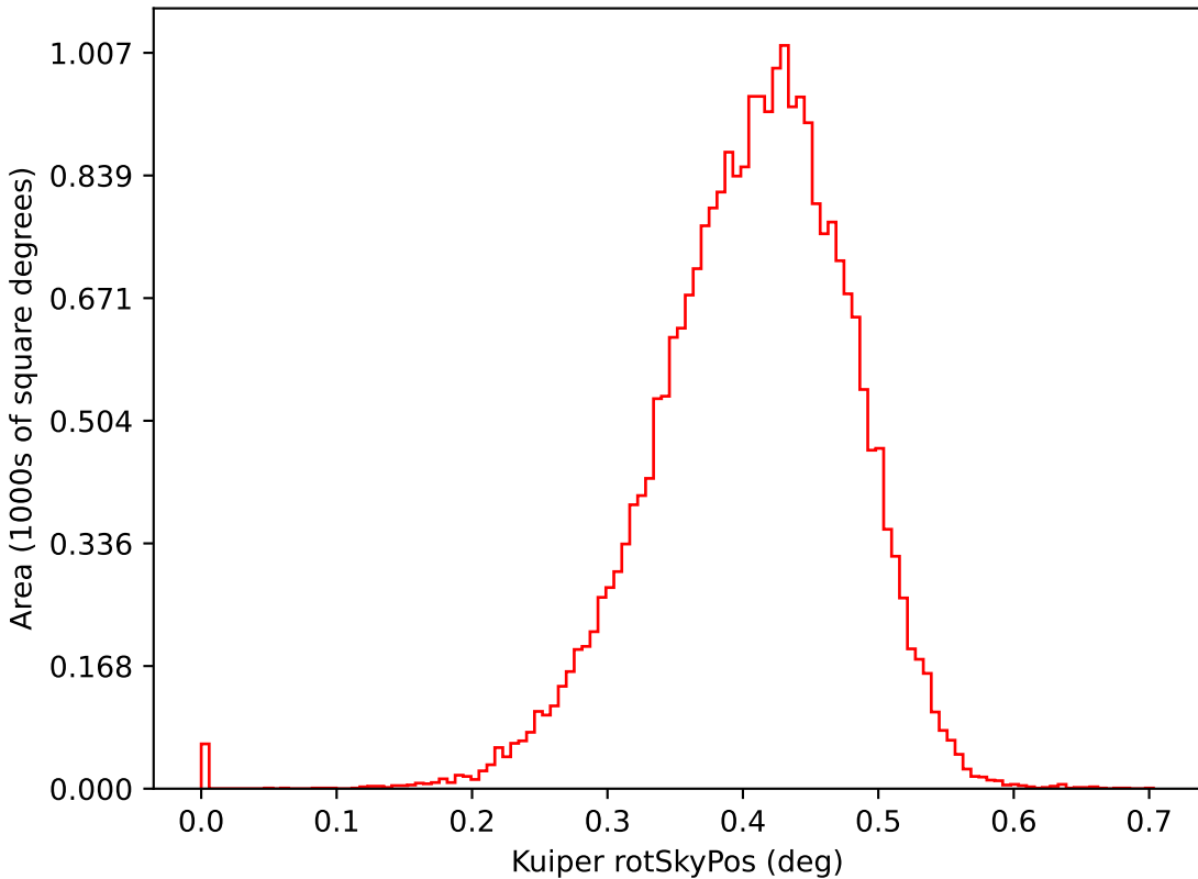
ddf_acor_sf25_ls30_lsr50_v3.4_10yrs i: Kuiper rotSkyPos
