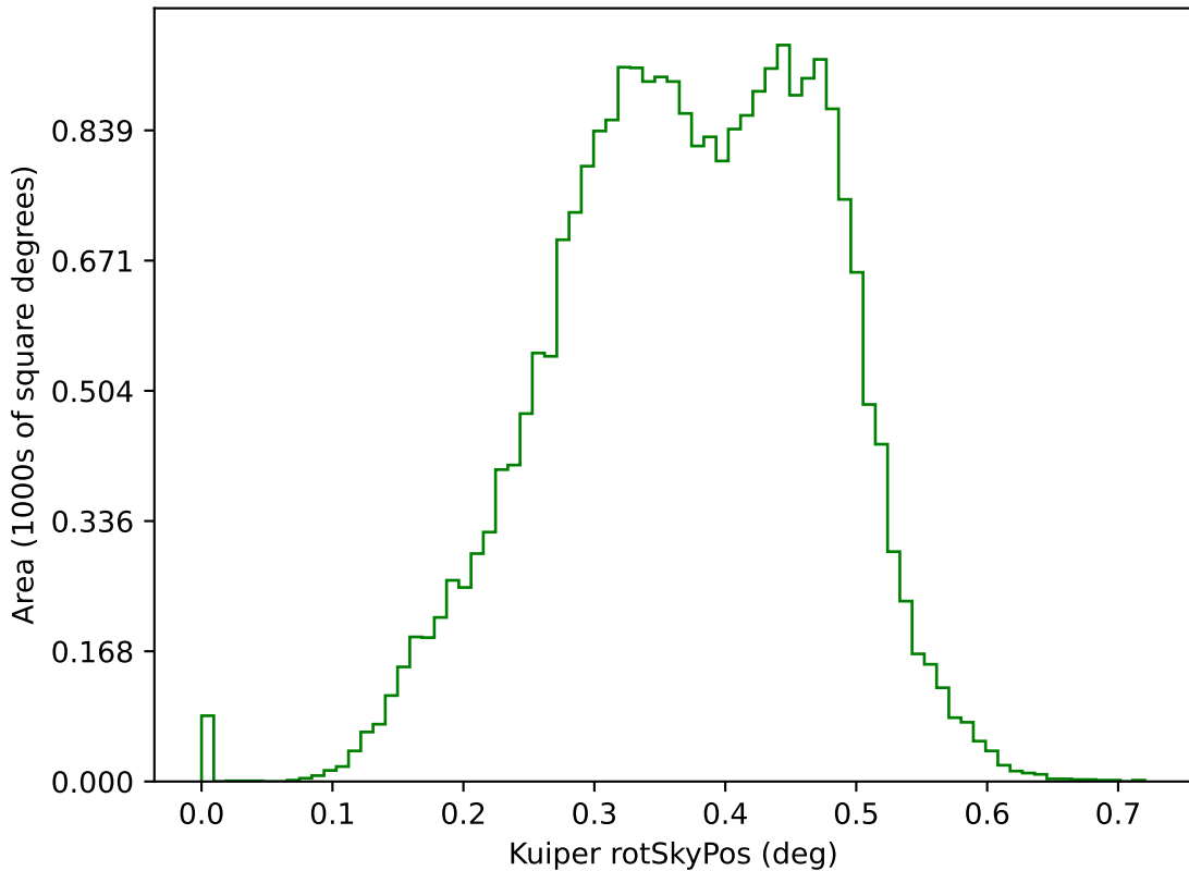
ddf_acor_sf25_lsf30_lsr50_v3.4_10yrs g: Kuiper rotSkyPos
