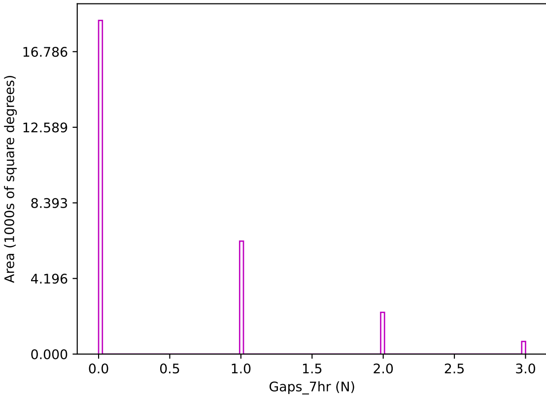
ddf_acor_sf25_ls30_lsr50_v3.4_10yrs z band: Gaps_7hr
