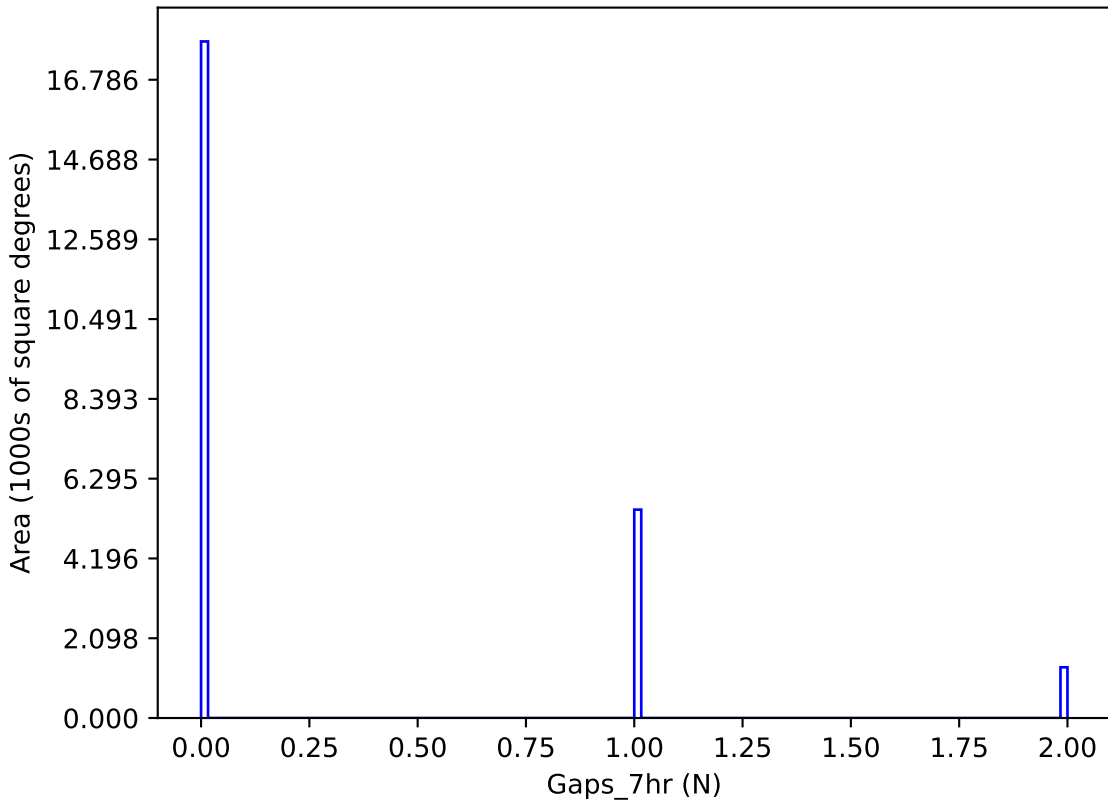
ddf_acor_sf25_lsf30_lsr50_v3.4_10yrs y band: Gaps_7hr
