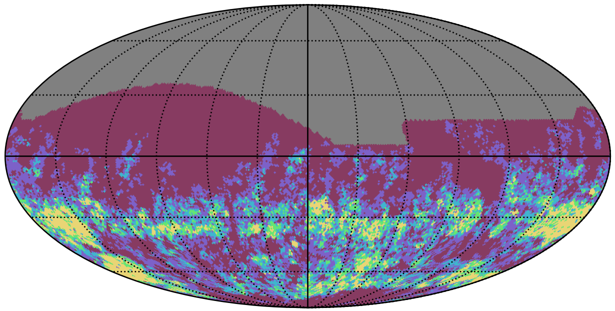
ddf_acor_sf25_lsf30_lsr50_v3.4_10yrs r band: Gaps_7hr
