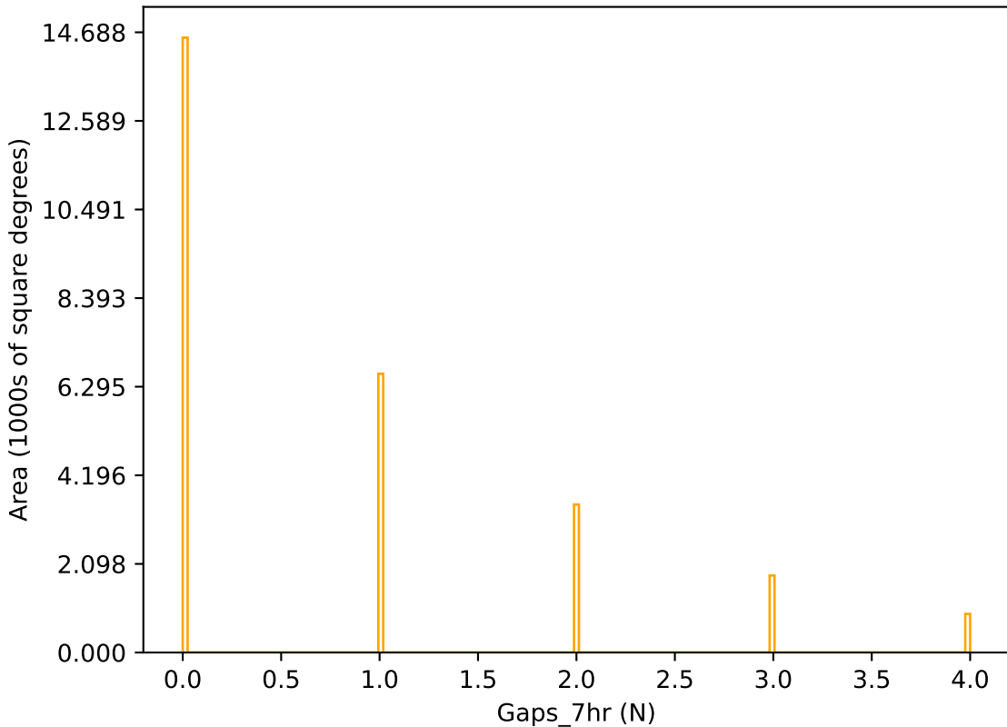
ddf_acor_sf25_lsf30_lsr50_v3.4_10yrs r band: Gaps_7hr
