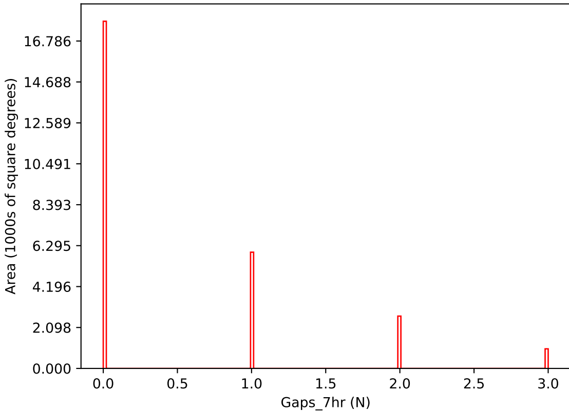
ddf_acor_sf25_lsf30_lsr50_v3.4_10yrs i band: Gaps_7hr
