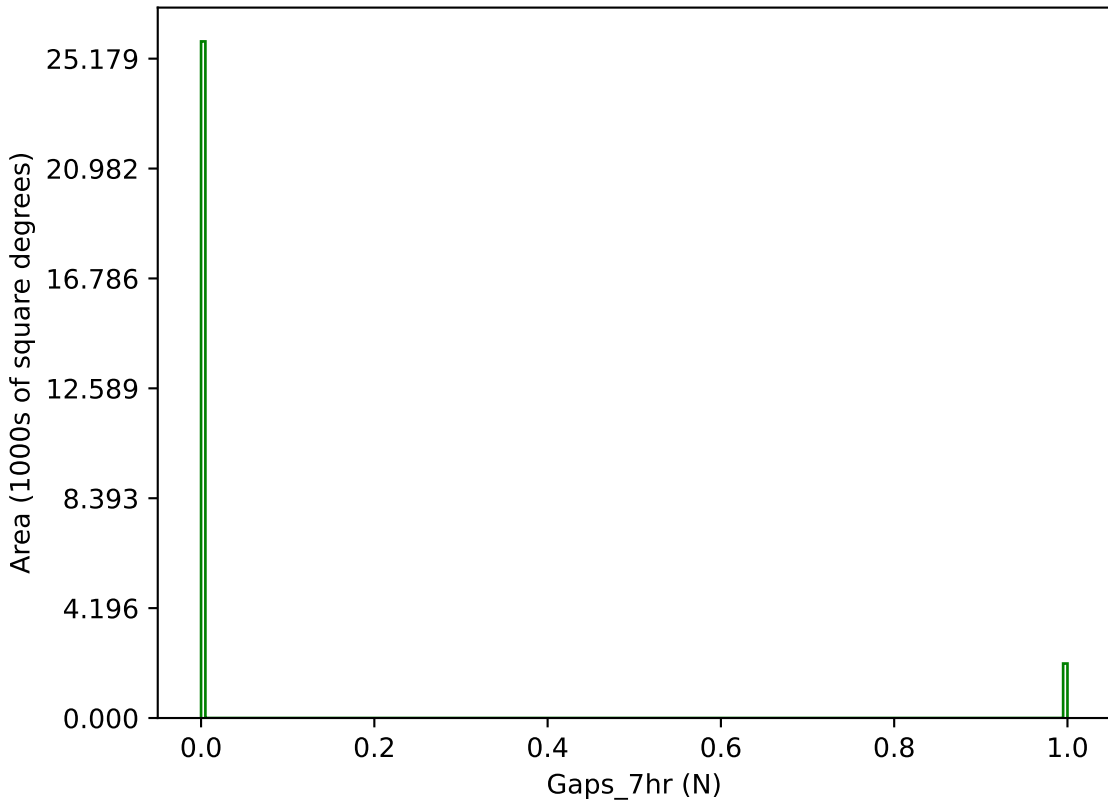
ddf_acor_sf25_lsf30_lsr50_v3.4_10yrs g band: Gaps_7hr
