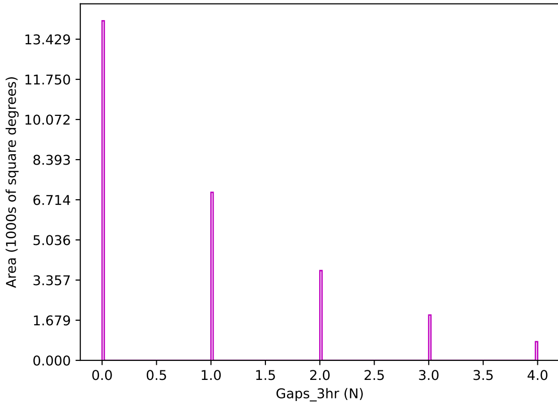
ddf_acor_sf25_lsf30_lsr50_v3.4_10yrs z band: Gaps_3hr
