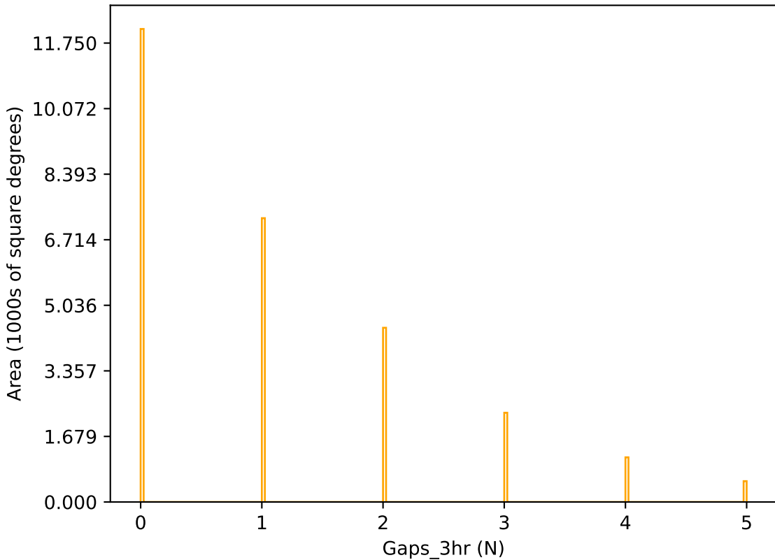
ddf_acor_sf25_lsf30_lsr50_v3.4_10yrs r band: Gaps_3hr
