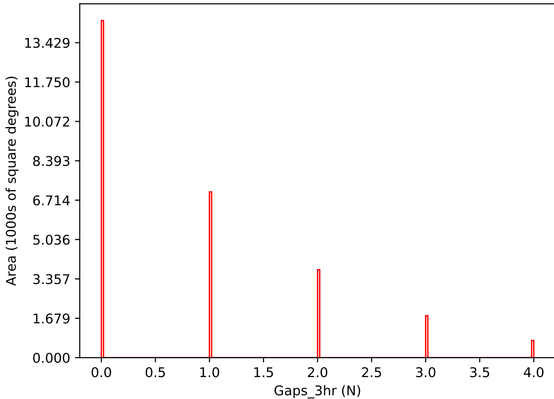
ddf_acor_sf25_lsf30_lsr50_v3.4_10yrs i band: Gaps_3hr
