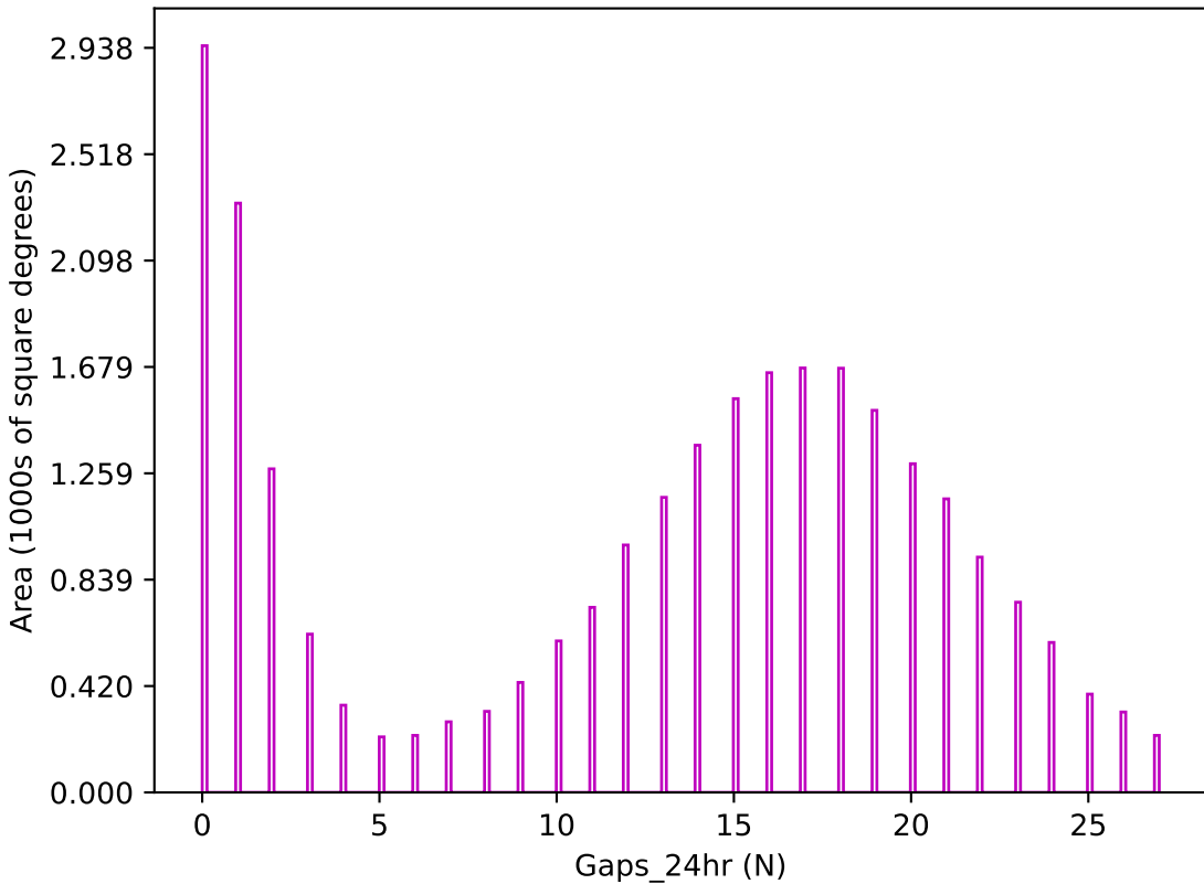
ddf_acor_sf25_lsf30_lsr50_v3.4_10yrs z band: Gaps_24hr
