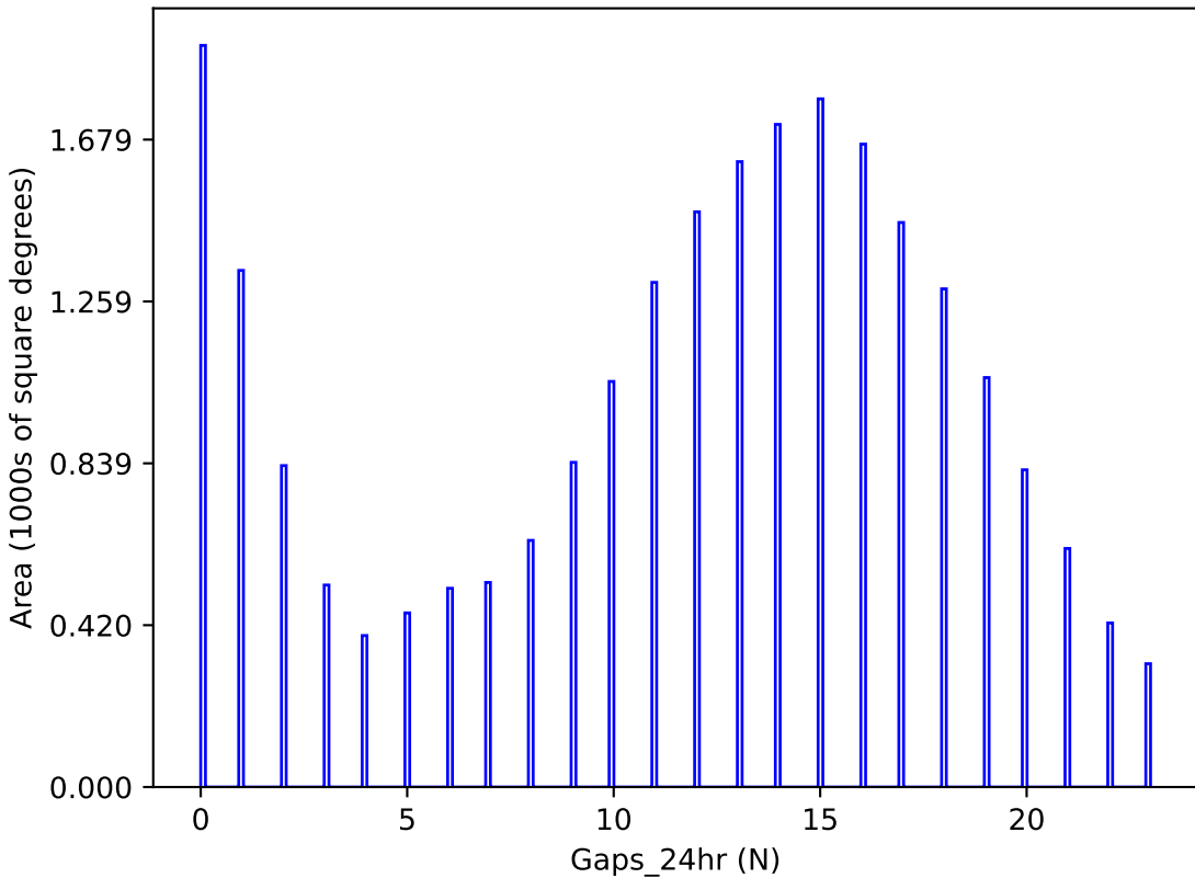
ddf_acor_sf25_lsf30_lsr50_v3.4_10yrs y band: Gaps_24hr
