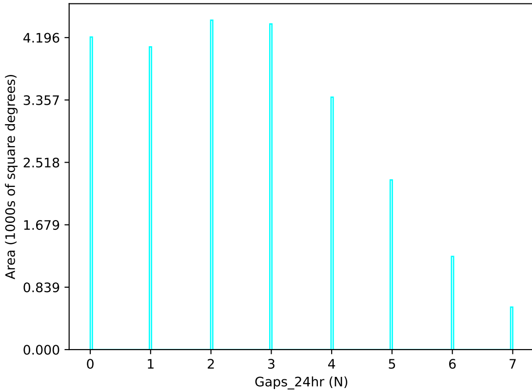
ddf_acor_sf25_lsf30_lsr50_v3.4_10yrs u band: Gaps_24hr
