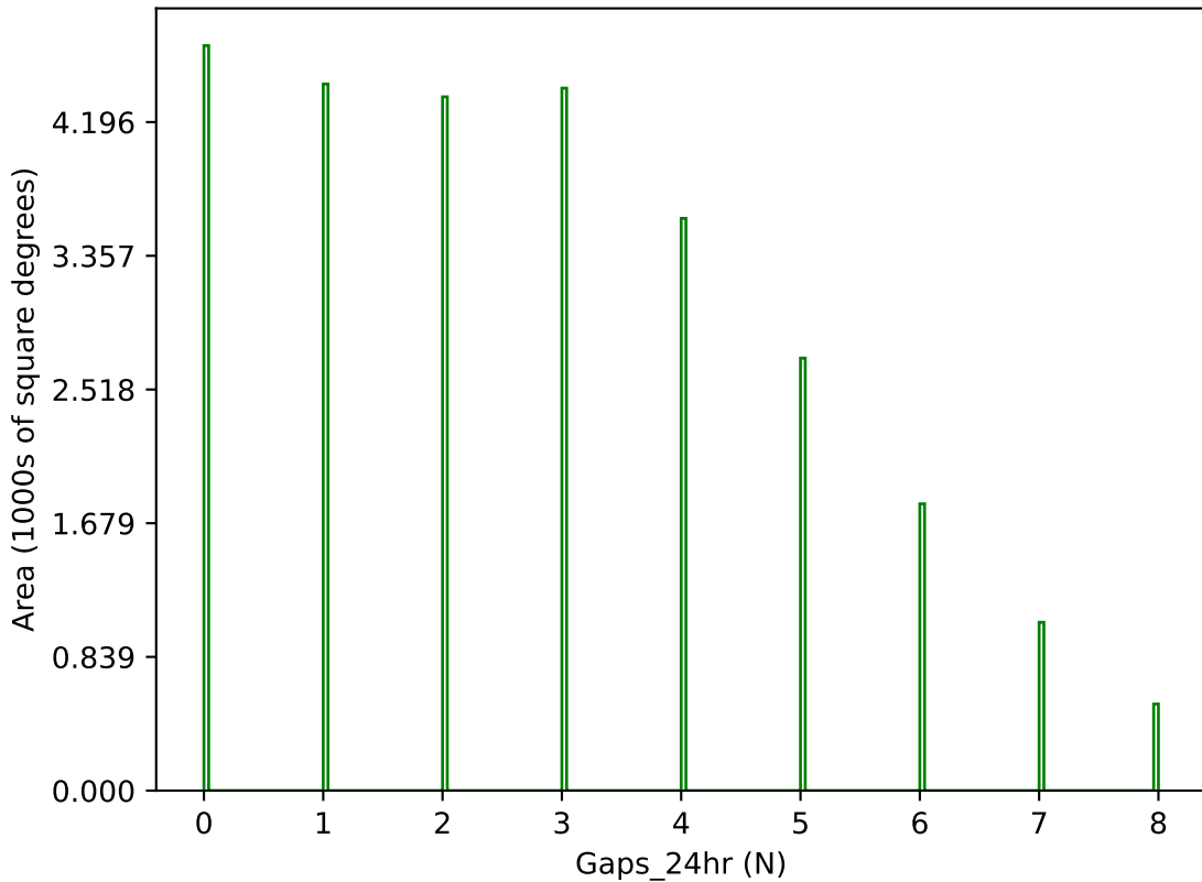
ddf_acor_sf25_lsf30_lsr50_v3.4_10yrs g band: Gaps_24hr
