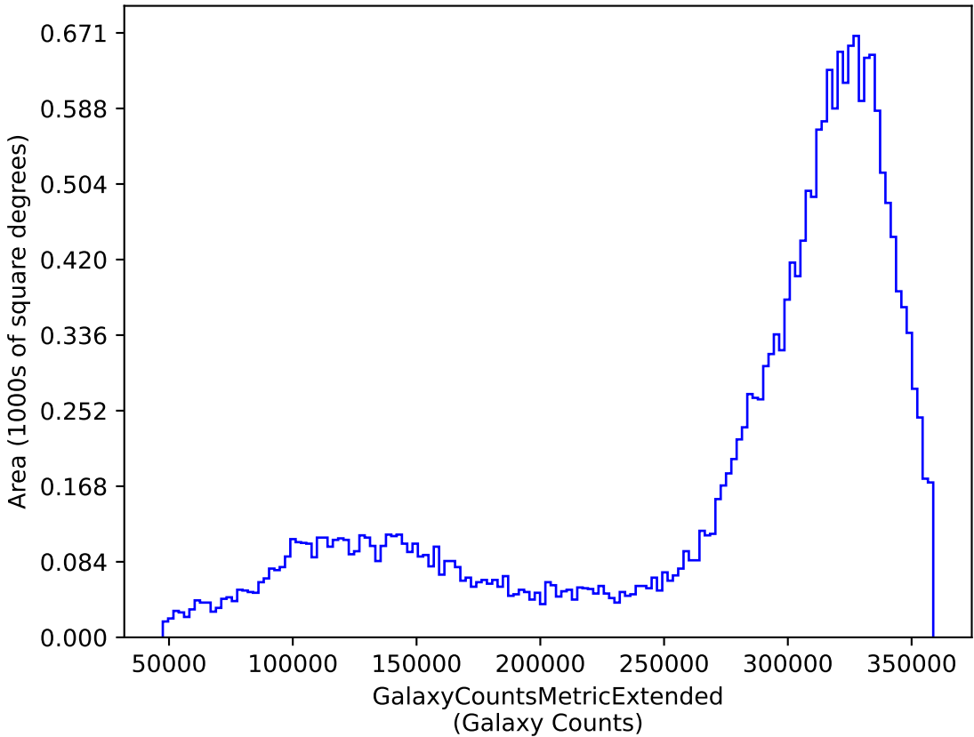
ddf_acor_sf25_lsf30_lsr50_v3.4_10yrs y: GalaxyCountsMetricExtended
