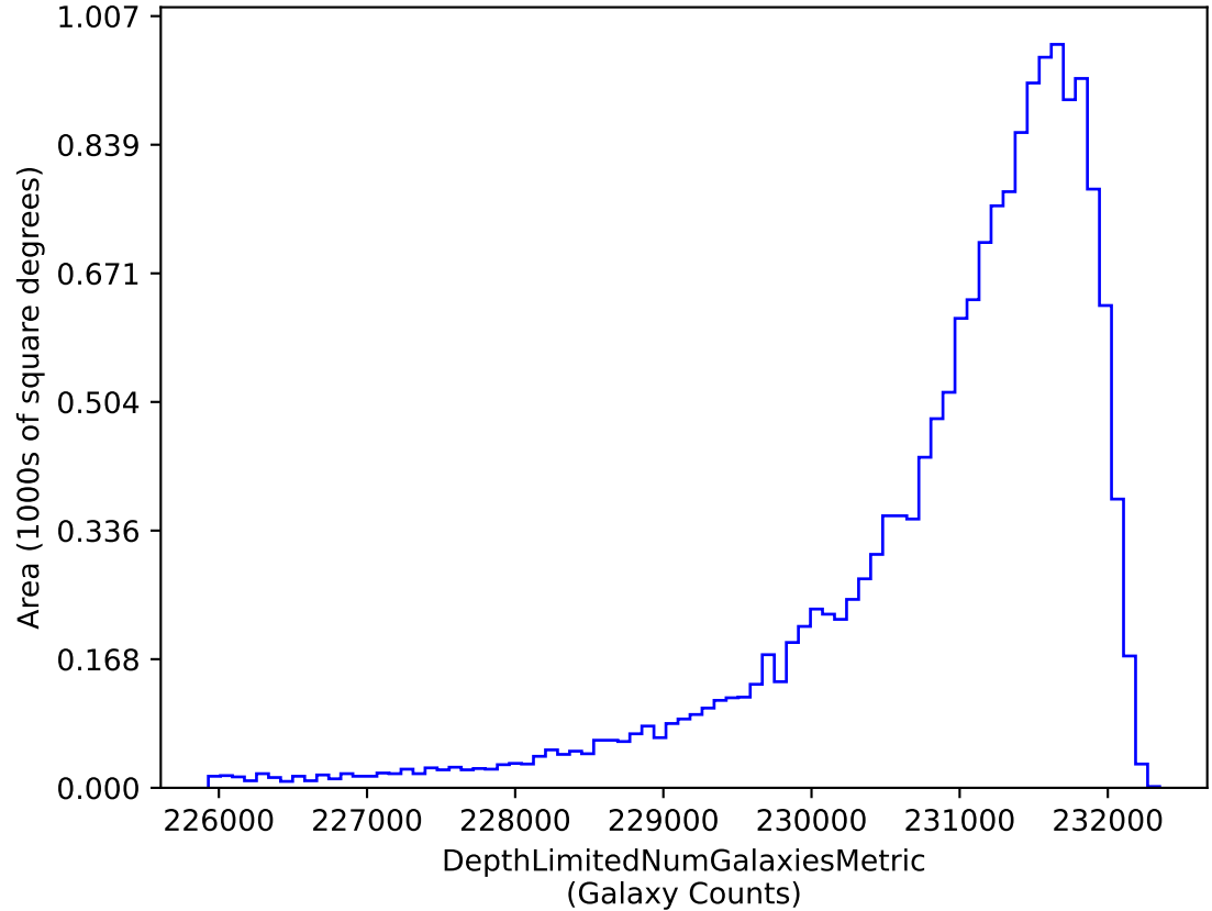
ddf_acor_sf25_lsf30_lsr50_v3.4_10yrs i band galaxies non-DD: DepthLimitedNumGalaxiesMetric
