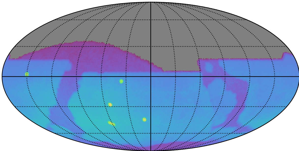
ddf_acor_sf25_lsf30_lsr50_v3.4_10yrs : Brown Dwarf, L7
