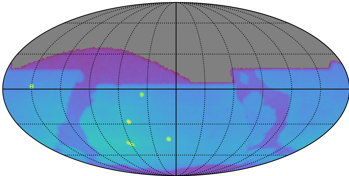
ddf_acor_sf25_lsf30_lsr50_v3.4_10yrs : Brown Dwarf, L4
