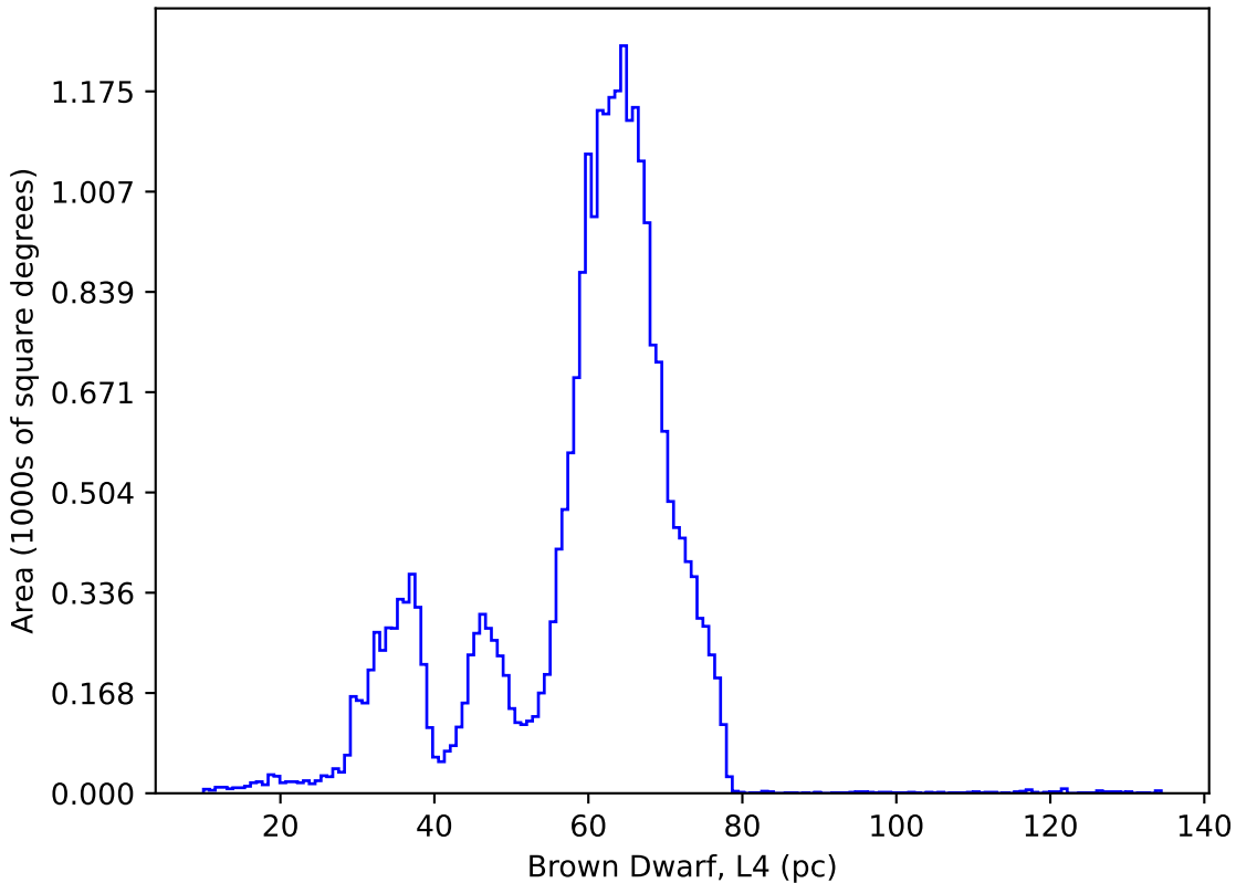
ddf_acor_sf25_lsf30_lsr50_v3.4_10yrs : Brown Dwarf, L4
