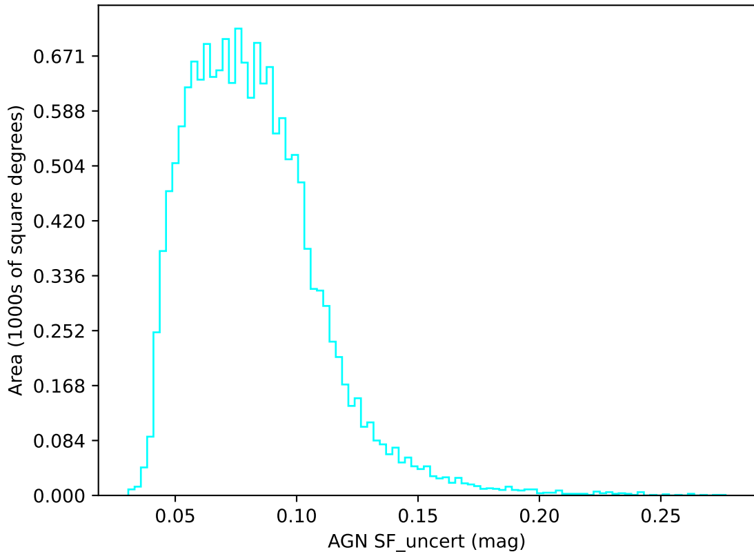
ddf_acor_sf25_lsf30_lsr50_v3.4_10yrs u band: AGN SF_uncert
