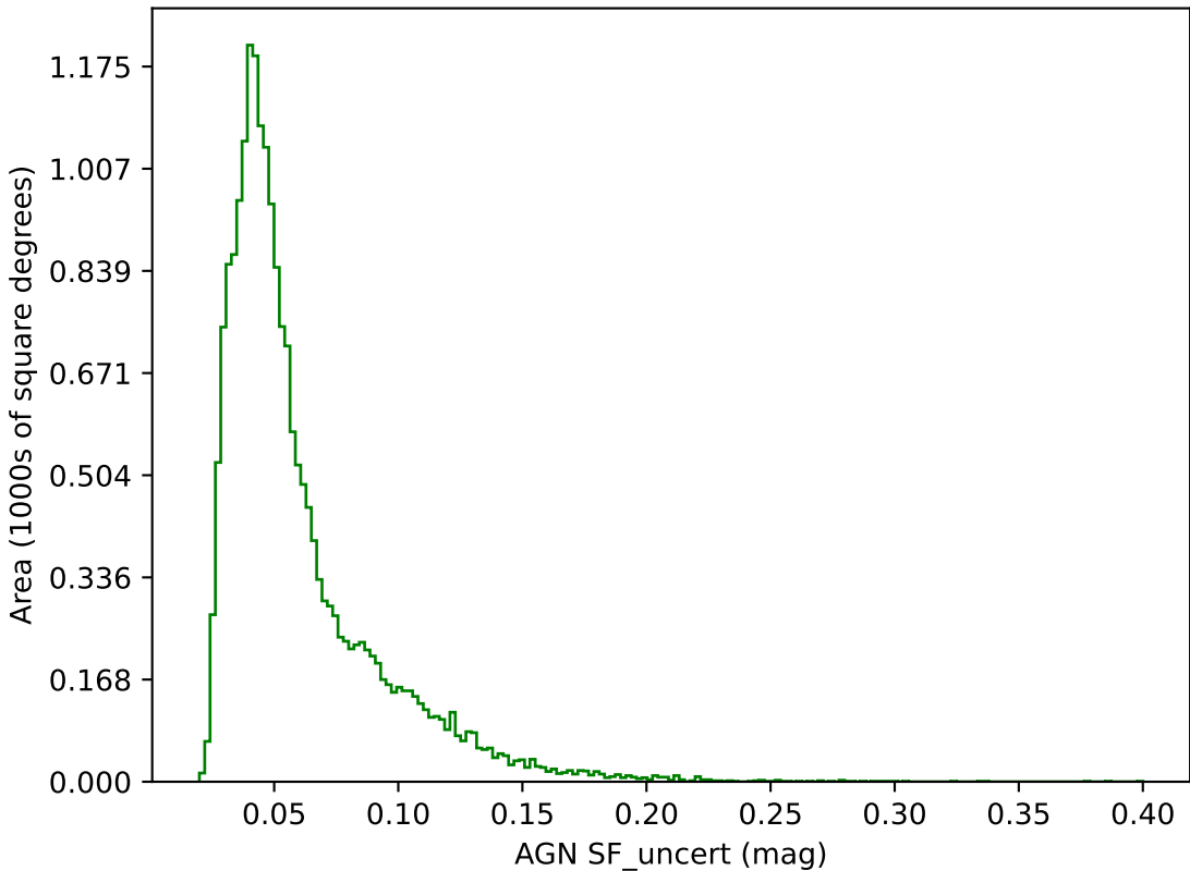
ddf_acor_sf25_lsf30_lsr50_v3.4_10yrs g band: AGN SF_uncert
