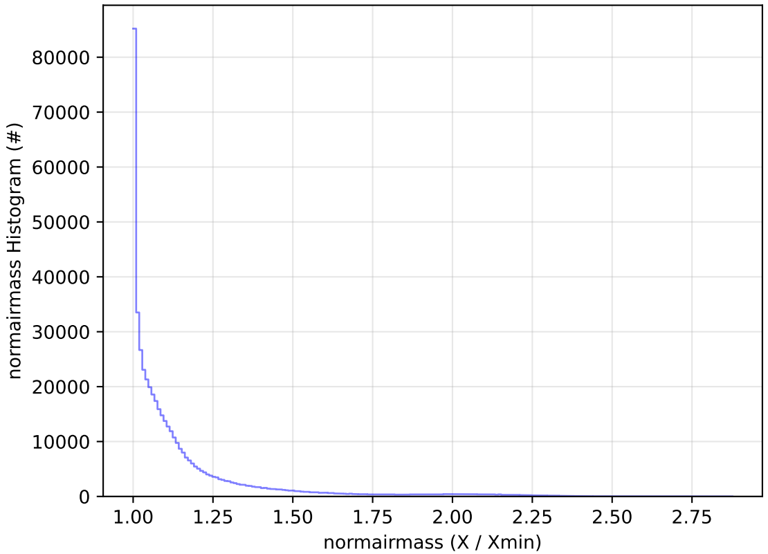
ddf_acor_sf25_lsf30_lsr50_v3.4_10yrs All sky r band: normairmass Histogram
