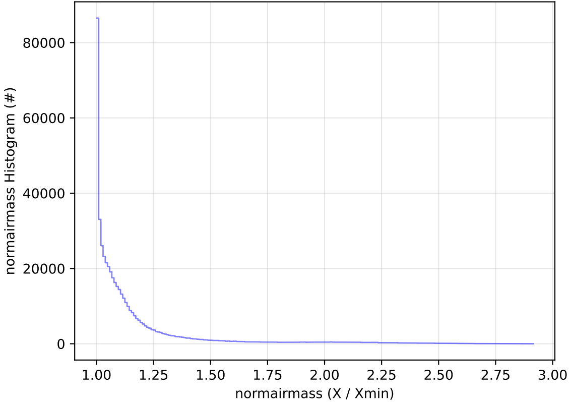
ddf_acor_sf25_lsf30_lsr50_v3.4_10yrs All sky i band: normairmass Histogram
