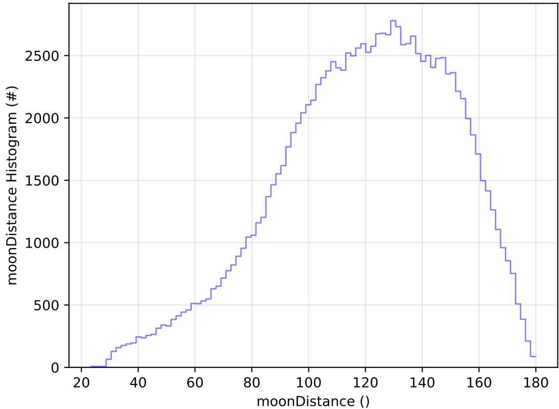
ddf_acor_sf25_lsf30_lsr50_v3.4_10yrs WFD u band: moonDistance Histogram
