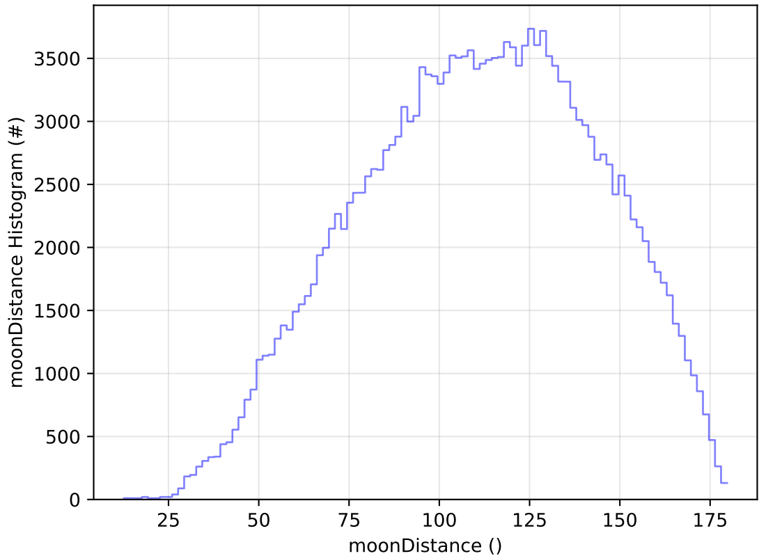
ddf_acor_sf25_lsf30_lsr50_v3.4_10yrs WFD g band: moonDistance Histogram
