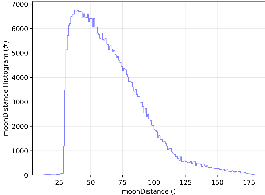
ddf_acor_sf25_lsf30_lsr50_v3.4_10yrs All sky y band: moonDistance Histogram
