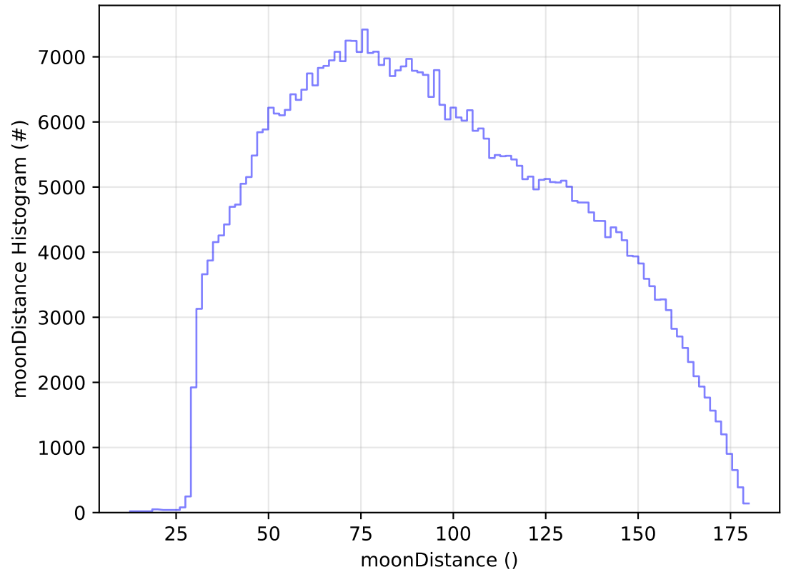
ddf_acor_sf25_lsf30_lsr50_v3.4_10yrs All sky i band: moonDistance Histogram
