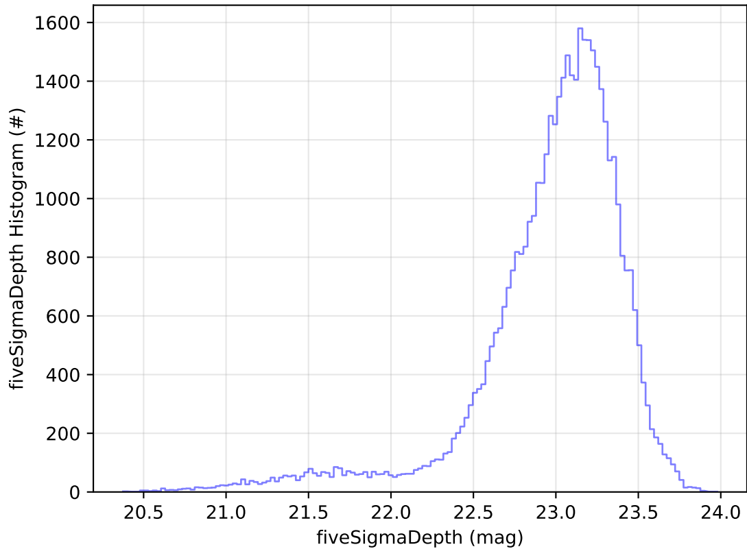
ddf_acor_sf25_lsf30_lsr50_v3.4_10yrs Yr 1 z band: fiveSigmaDepth Histogram
