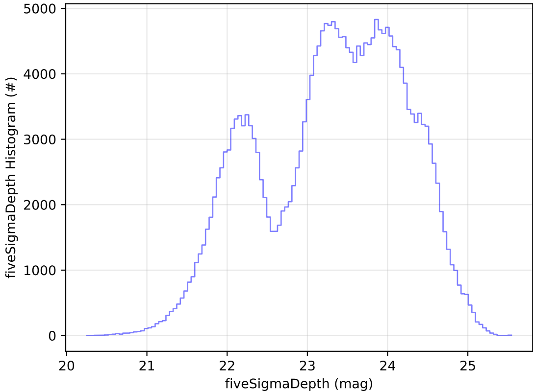
ddf_acor_sf25_lsf30_lsr50_v3.4_10yrs Yr 1 all bands: fiveSigmaDepth Histogram
