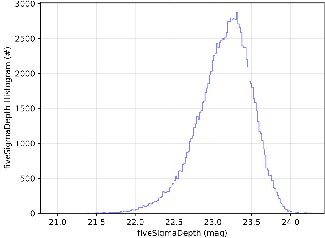
ddf_acor_sf25_lsf30_lsr50_v3.4_10yrs All sky u band: fiveSigmaDepth Histogram
