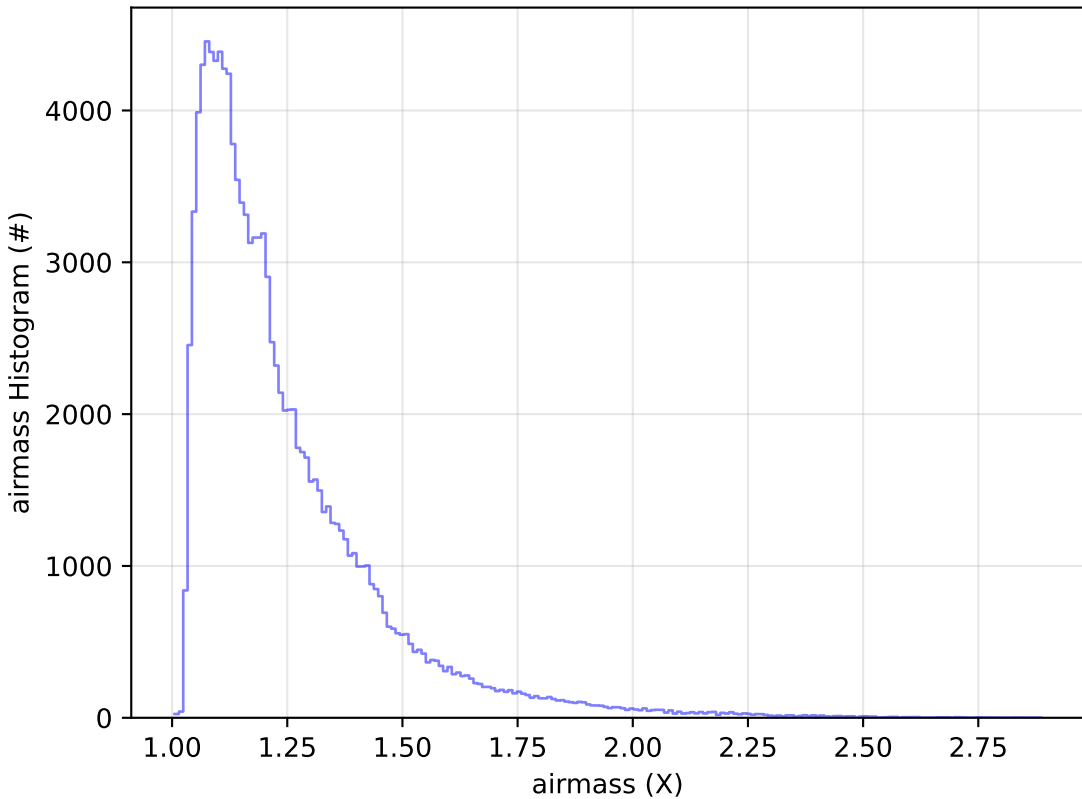
ddf_acor_sf25_lsf30_lsr50_v3.4_10yrs WFD u band: airmass Histogram
