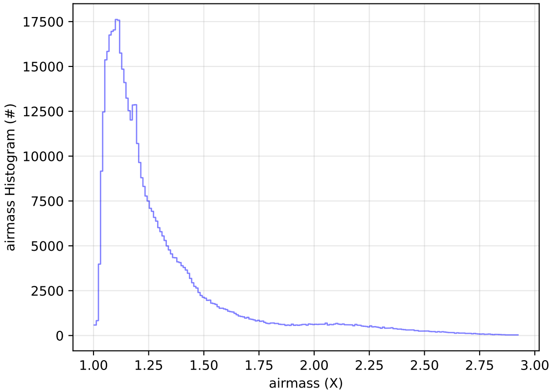
ddf_acor_sf25_lsf30_lsr50_v3.4_10yrs All sky i band: airmass Histogram
