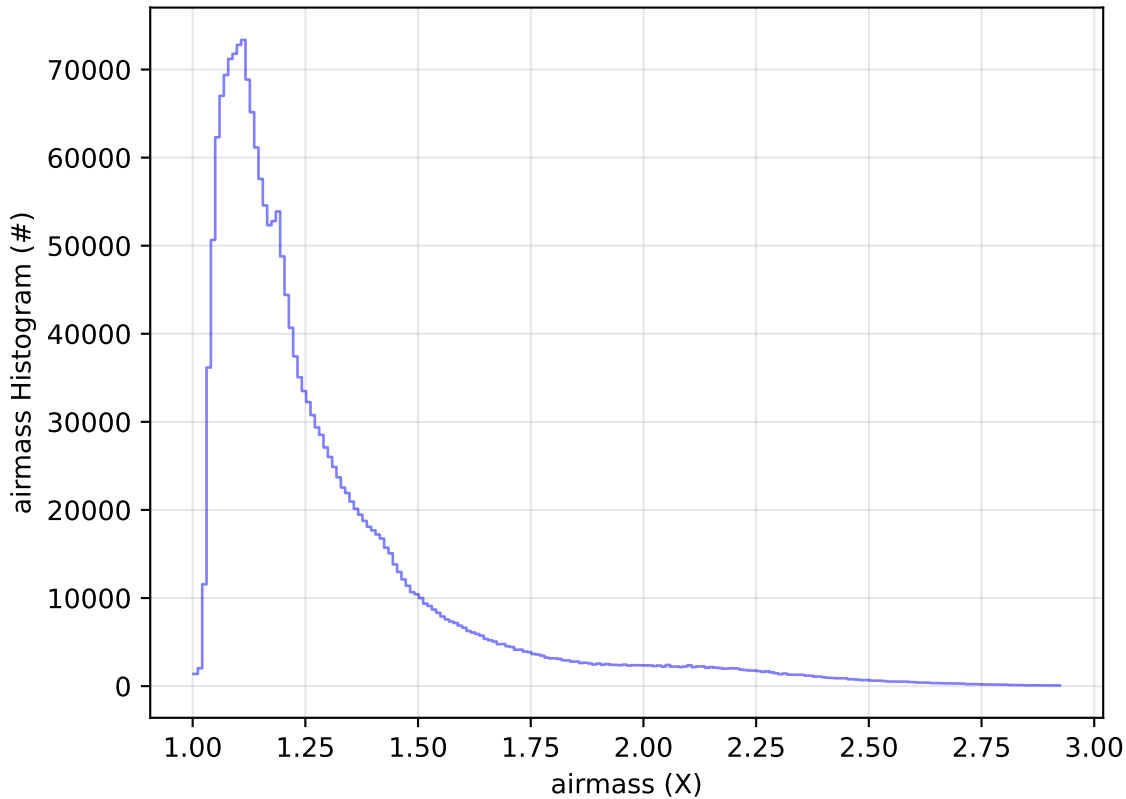
ddf_acor_sf25_lsf30_lsr50_v3.4_10yrs All sky all bands: airmass Histogram
