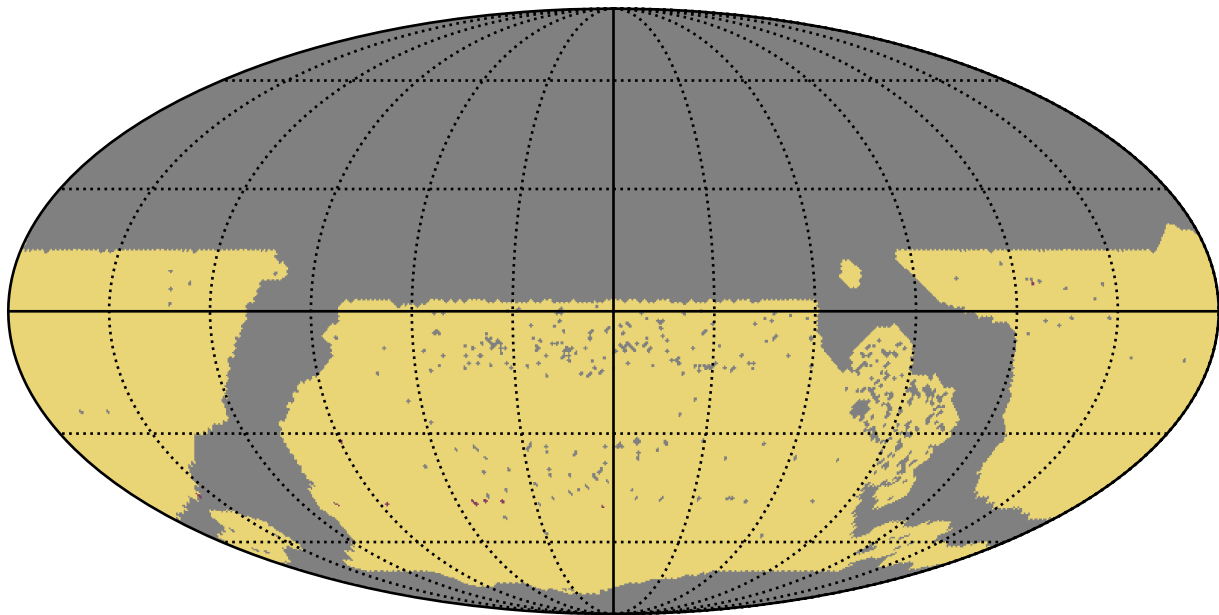
ddf_acor_sf25_lsf30_lsr50_v3.4_10yrs WFD: RapidRevisits
