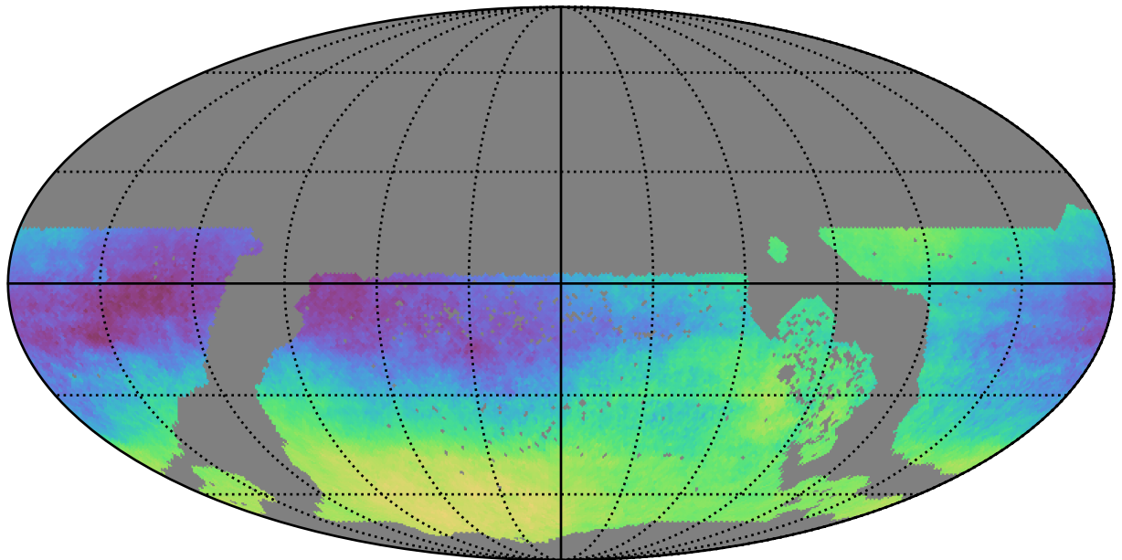
ddf_acor_sf25_lsf30_lsr50_v3.4_10yrs WFD: Parallax-DCR degeneracy @ 24.0
