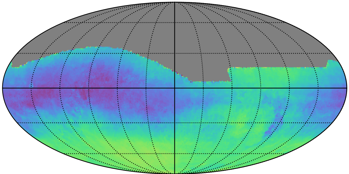
ddf_acor_sf25_lsf30_lsr50_v3.4_10yrs All sky: Parallax-DCR degeneracy @ 24.0
