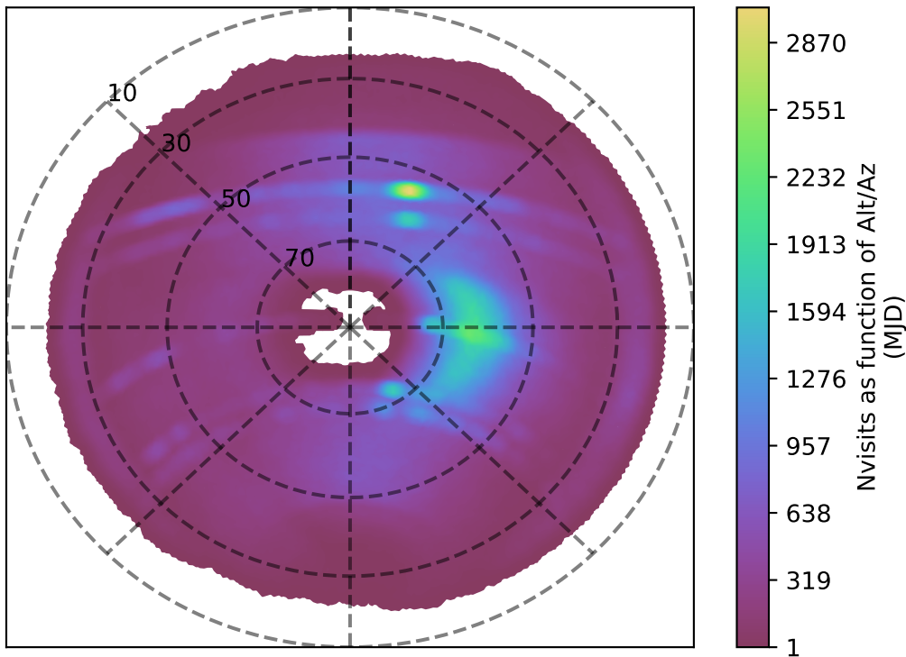
ddf_acor_sf25_lsf30_lsr50_v3.4_10yrs z band: Nvisits as function of Alt/Az
