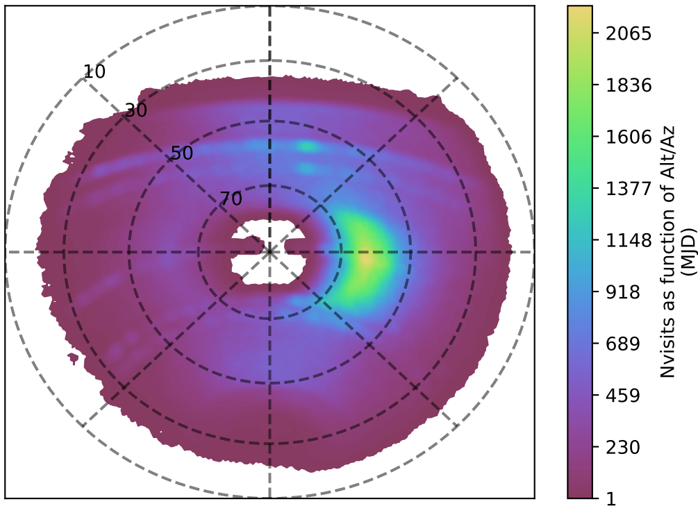
ddf_acor_sf25_lsf30_lsr50_v3.4_10yrs y band: Nvisits as function of Alt/Az
